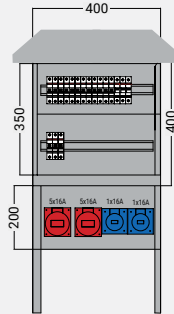
Pano Tipi/ Pano Kodu: Panel Type/Panel Code: TIP-1/ POK SP 754030
