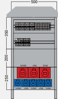
Pano Tipi/ Pano Kodu: Panel Type/Panel Code: TIP-2/ POK SP 1005030
